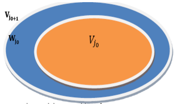
Fig 1: Orthogonal Decomposition of Space
