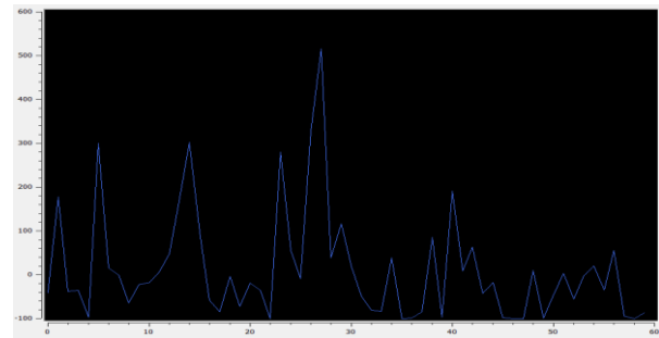
Fig 4: Wavelet Decomposition of Percentage Departure of Rainfall
