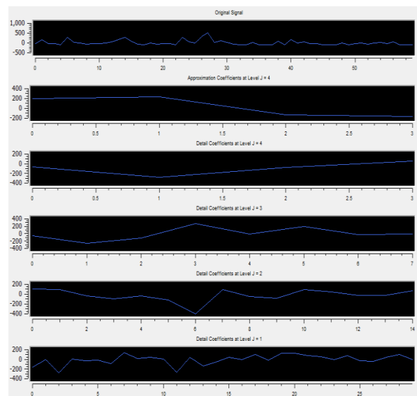
Fig 4: Wavelet Decomposition of Percentage Departure of Rainfall
