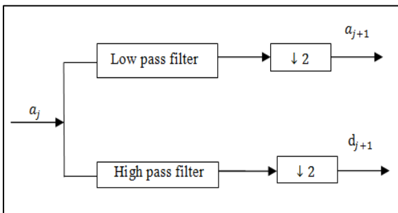
Fig 2: Decomposition of wavelet coefficients
